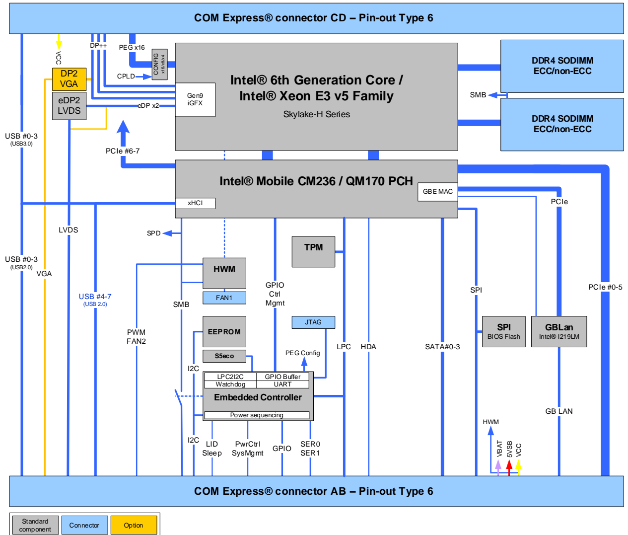
Figure 1: Block Diagram COMe-bSL6
