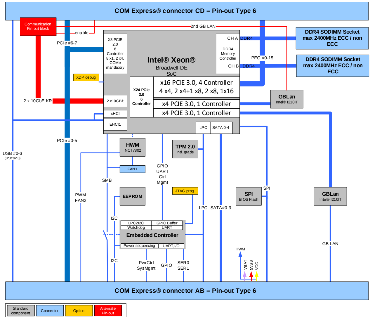
Figure 1: Block Diagram COMe-bBD6
