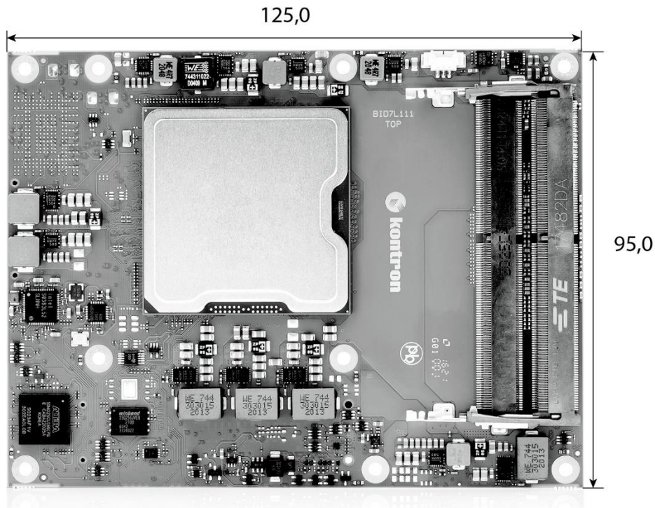
Figure 5: Module Dimensions
