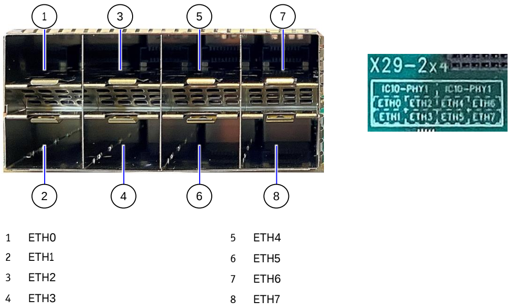
Figure 20: Side View of 2x4 SFP28 Cage (X29)
