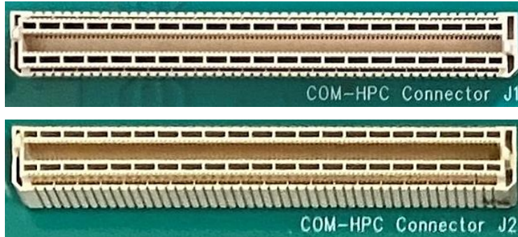
Figure 43: COM-HPC Connector J1 and J2
